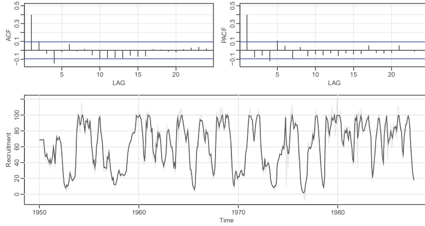
Fig. 5.12. Top: ACF and PACF of the estimated noise u_t . Bottom: The recruitment series (line) and the one-step-ahead predictions (gray swatch) based on the final transfer function model.
