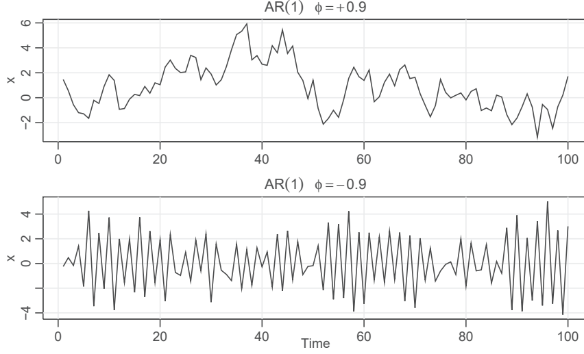
Fig. 3.1. Simulated AR(1) models: \phi = .9 (top); \phi = -.9 (bottom).
