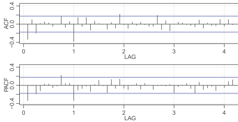
Fig. 3.23. Sample ACF and PACF of ddx ( \nabla_{12}\nabla \log x_t ).
