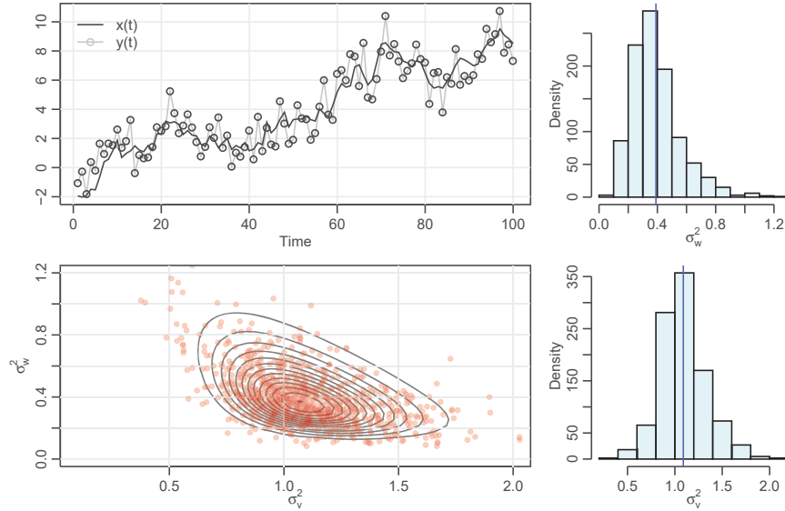
Fig. 6.20. Display for Example 6.26 : Left: Generated states, x_t and data y_t . Contours of the likelihood (solid line) of the data and sampled posterior values as points. Right: Marginal sampled posteriors and posterior means (vertical lines) of each variance component. The true values are \sigma_w^2 = .5 and \sigma_v^2 = 1 .
