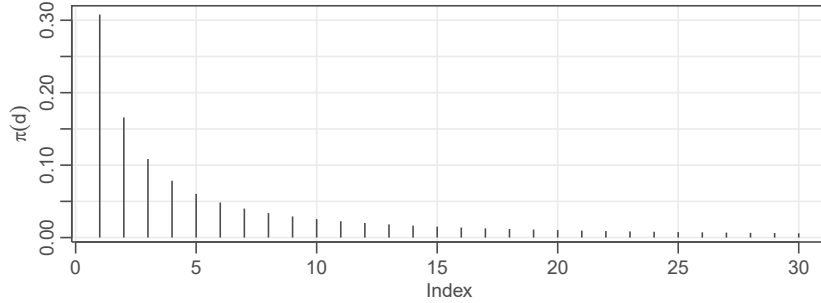
Fig. 5.2. Coefficients \pi_j(.384) , j = 1, 2, \dots, 30 in the representation (5.7).
