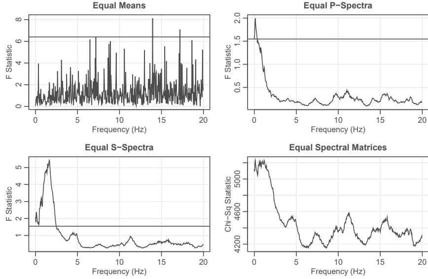
Fig. 7.11. Tests for equality of means, spectra, and spectral matrices for the earthquake and explosion data p = 2, L = 21, n = 1024 points at 40 points per second.
