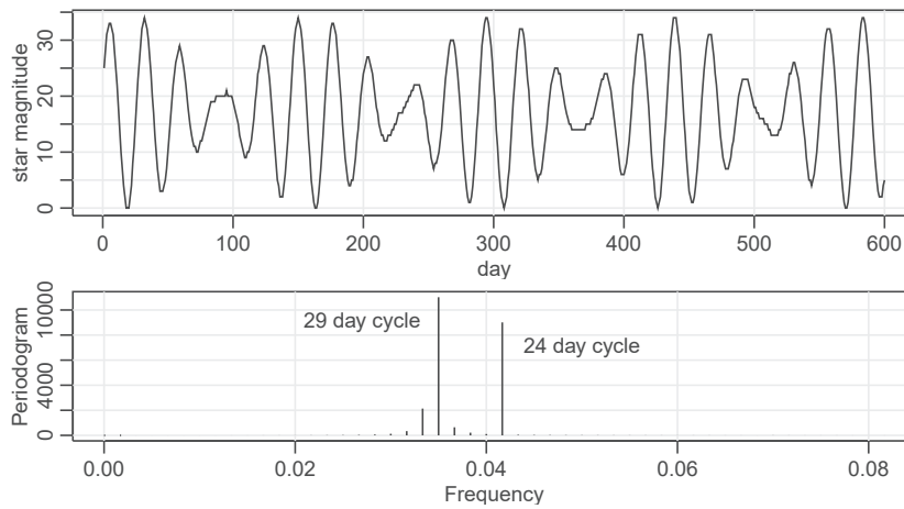
Fig. 4.3. Star magnitudes and part of the corresponding periodogram.
